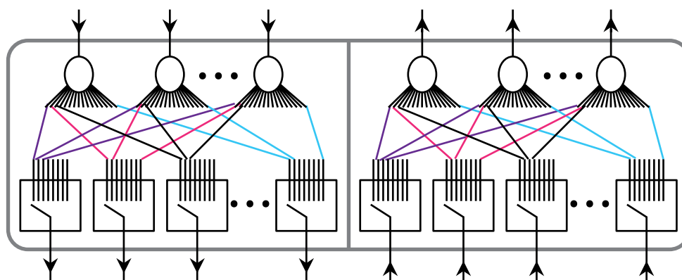
Twin NxM MCS with control circuit
